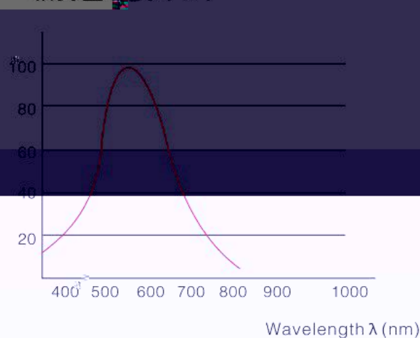
Spectrum Response Characteristic. 光譜回應特性曲線
